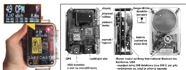
Fig. 2. Equipment for mobile monitoring.
