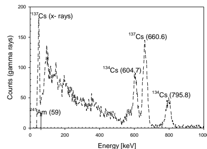
Fig. 1. 134,137 Cs spectra as detected by the GeoMAREA system (Tsabaris et al., 2019)
