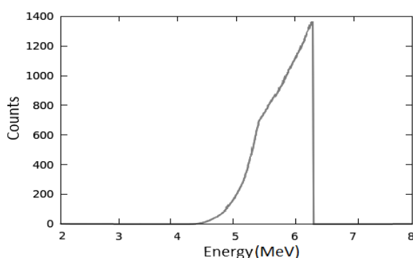
Figure 1. \alpha -spectrum of ^{220}\text{Rn} nuclei at 6.3 MeV obtained from the silicon detector inside the small Thoron chamber, using a Monte Carlo simulation.
