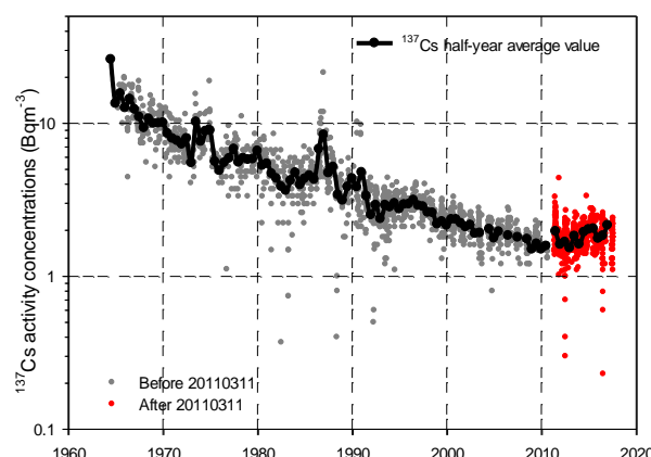
Figure 1. Temporal variations of ^{137}\text{Cs} concentrations in the SOJ. Red circle is measured after FNPP1 accident.
