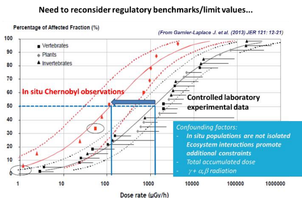
Figure 2. Mismatch between controlled laboratory experiments and field data obtained in Chernobyl contaminated territories
