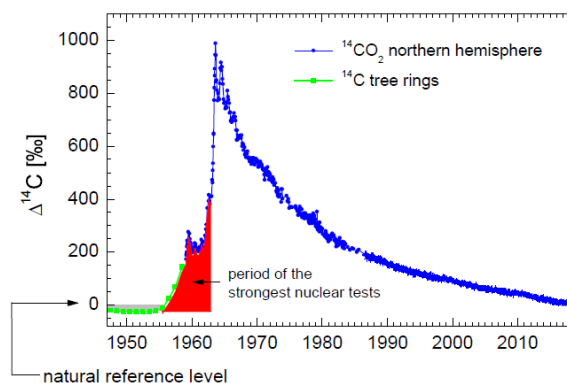
Figure 1: Long-term development of the 14 C/C ratio in atmospheric CO 2 in the Northern Hemisphere given as permil-deviation from an internationally accepted reference material. Zero Δ 14 C approximately corresponds to the natural 14 C/C ratio in atmospheric CO 2 , i.e. the equilibrium value between production in the upper atmosphere and decay in all carbon compartments.
