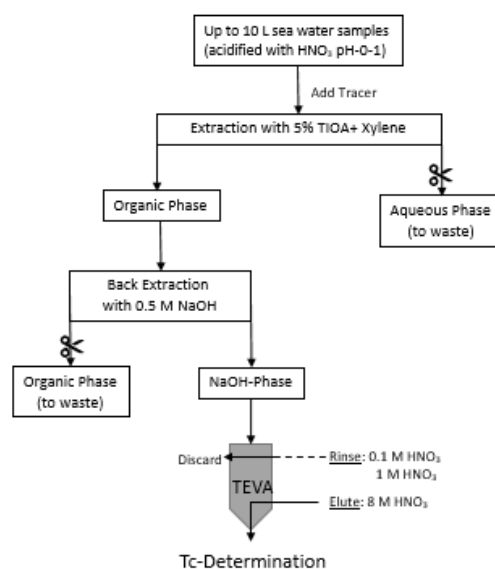
Figure-1. Chemical process for Tc preconcentration and purification
