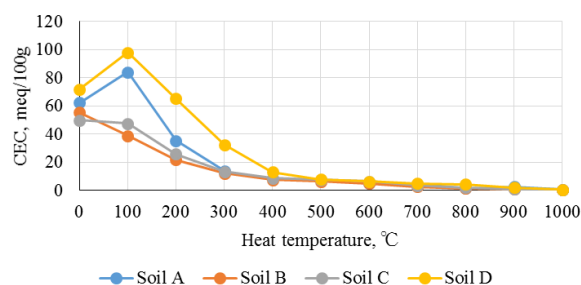
Figure 1. CEC of the heated soil.
