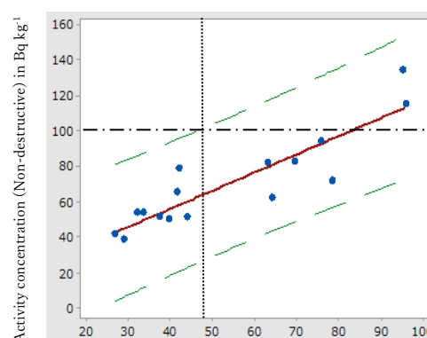
Fig.1 The regression line obtained with the present measurements using the WSI and the Ge detector.
