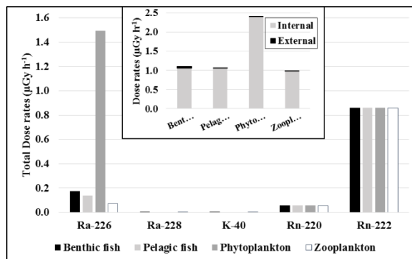
Figure 1. Dose rate assessment of marine biota at a submarine groundwater discharge, utilizing in situ gamma-ray measurements of KATERINA and GeoMAREA detectors
