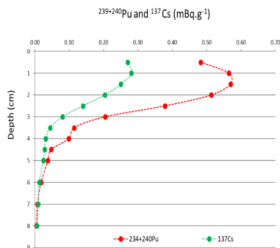
Figure 1. Profiles of ^{137}\text{Cs} and ^{239+240}\text{Pu} in sediment core
