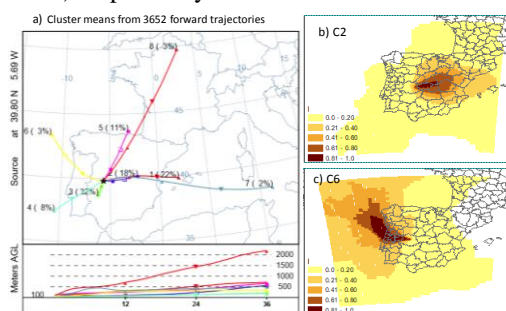
Figure 1. a) Mean cluster pathways (centroids).
