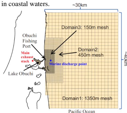
Figure 1. Simulation domain of the coastal marine model for the Rokkasho coast.
