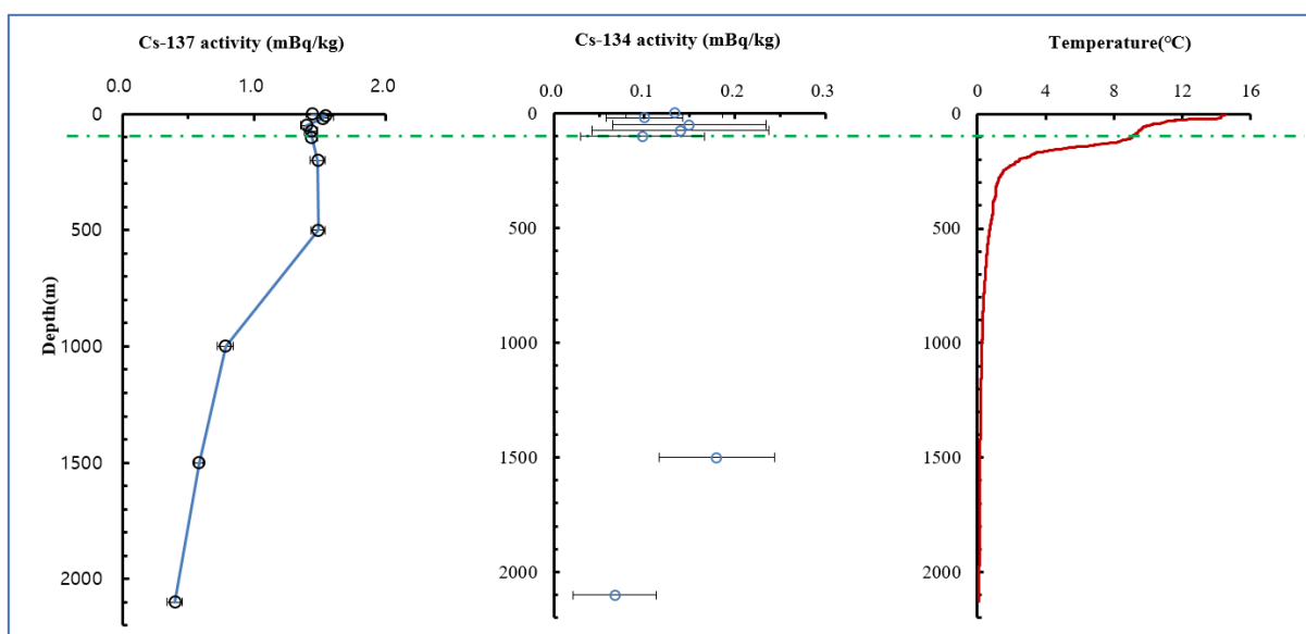
Figure 1 Vertical profiles of ^{134}\text{Cs} and ^{137}\text{Cs} activity concentration and water temperature at Stn. M (2011-06-01) in the Uleung Basin in the East Sea/Sea of Japan.
