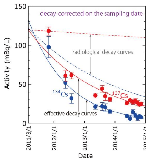
Figure 1. Temporal changes in the contents of radioactive cesium in Yugama water.
