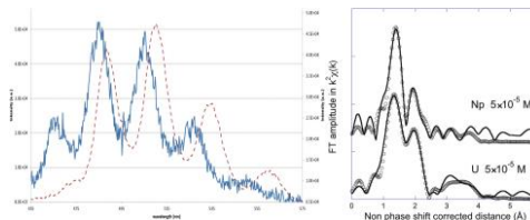
Figure 1 TRLIF and EXAFS spectra of U in seawater, \text{UO}_2(\text{CO}_3)_3\text{Ca}_2 (plain curve), \text{UO}_2^{2+} (dotted line)
