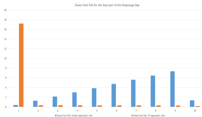
Figure 2. Comparison of doses to human from ^{137}\text{Cs} in fish for the Stepovogo Bay, mSv
