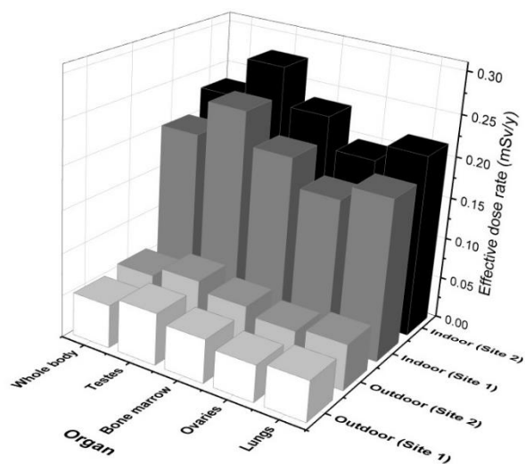
Figure 2. the effective dose rate delivered to the particular organs (Lungs, Ovaries, Bone marrow, Testes and Whole body) from air dose indoor and outdoor.
