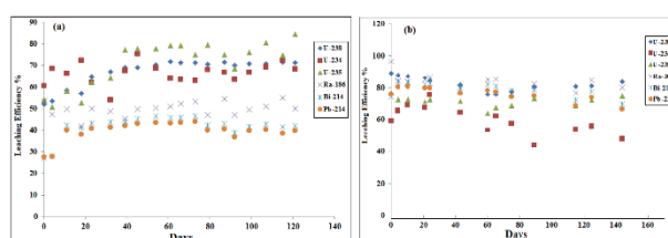
Figure 1. Leaching efficiency of Uranium isotopes in (a) pregnant solution and (b) total solution.
