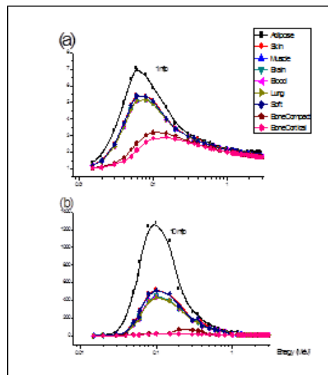
Figure 1. The exposure build-up factor for; adipose, skin, muscle, brain, blood, lung, soft, bone (compact), and bone (cortical) tissues in the energy region 0.015 – 3 MeV at (a) 1 mfp, (b) 10 mfp.
