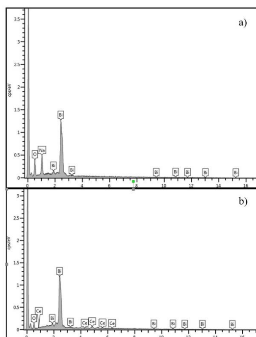
Figure 2 EDS spectrum of (a) as-prepared NaBiO 3 and (b) after Ce 3+ adsorption.
